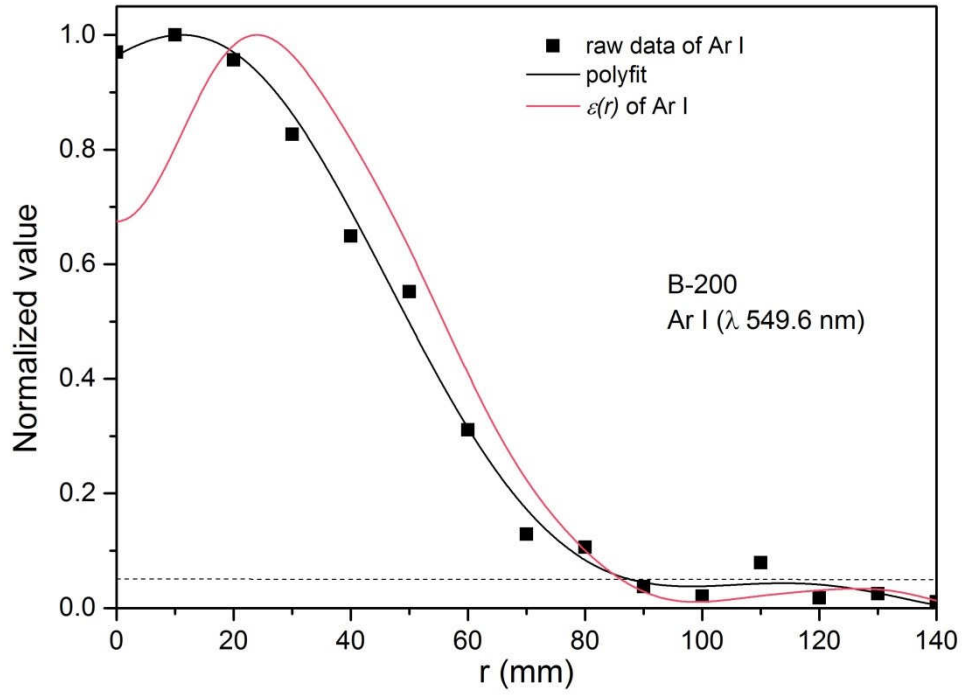
Fig. 5 Radial profile of measured intensities I(y) , polynomial fits of raw data and the reconstructed emissivities \varepsilon(r) of Ar I line (549.6 nm) under condition B-200 (Ar/He/H 2 jet, 200 Pa); The dashed line describes the 5% level of the normalized value
